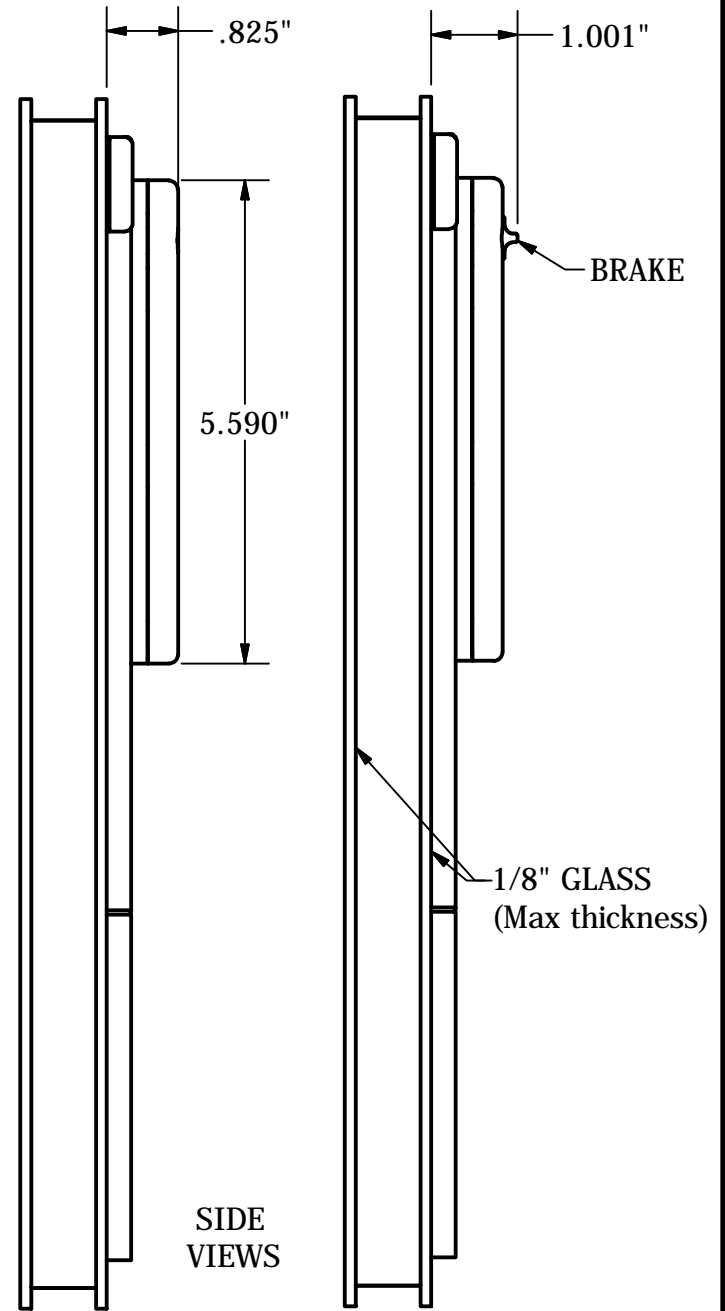
WITHOUT BRAKE
